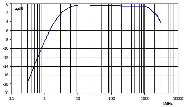
TYPICAL RESPONSE SMT2-0005
