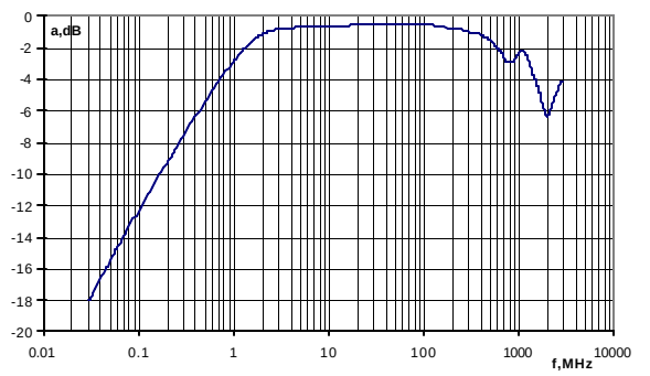
TYPICAL RESPONSE SMT2-0007
