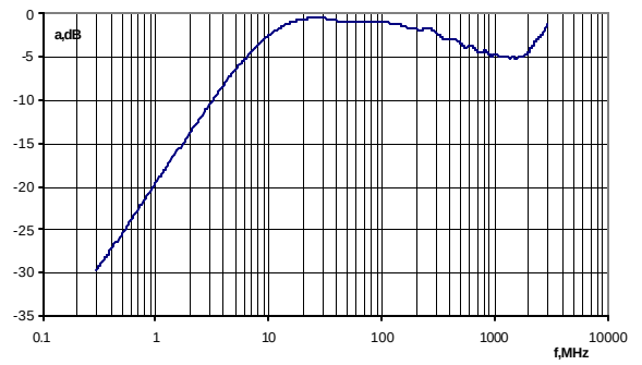
TYPICAL RESPONSE SMT2-0001
