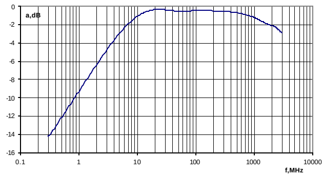
TYPICAL RESPONSE SMT2-0010
