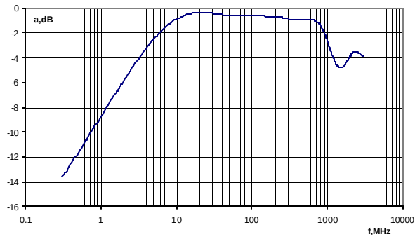
TYPICAL RESPONSE SMT2-0000
